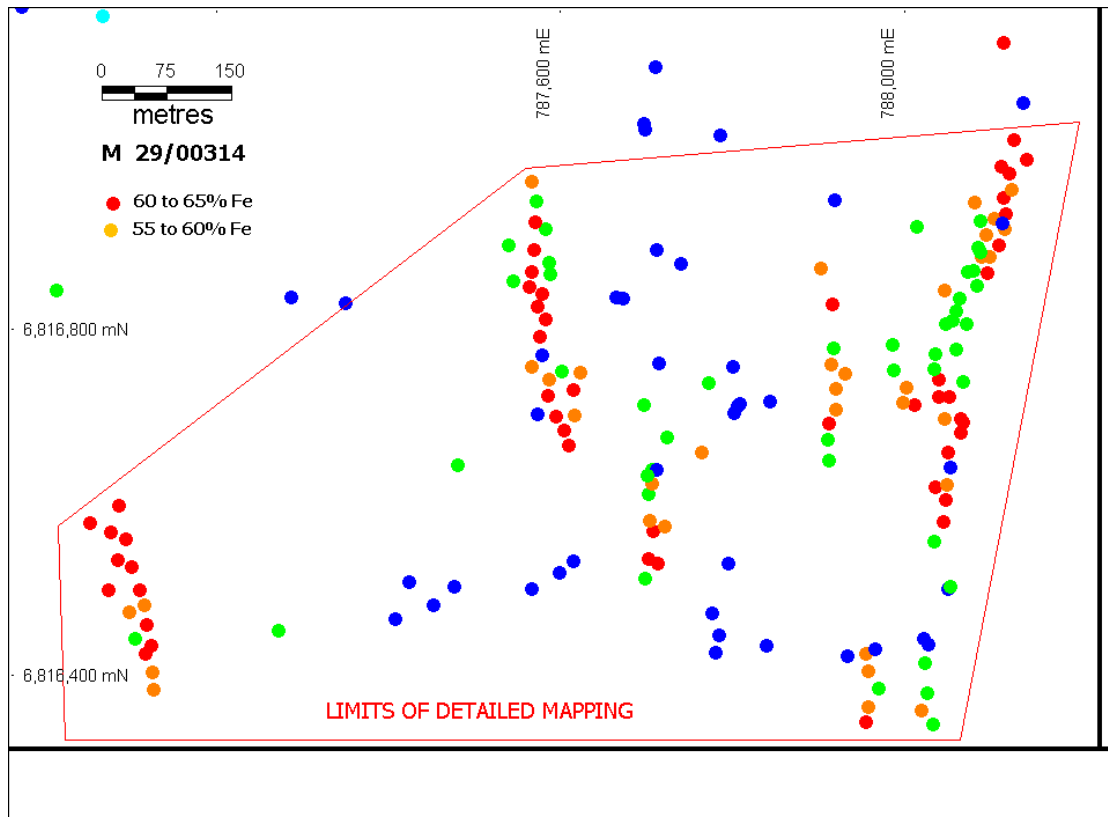
Figure 1 - Distribution of Rock Chip Sampling – Mt Forrest
